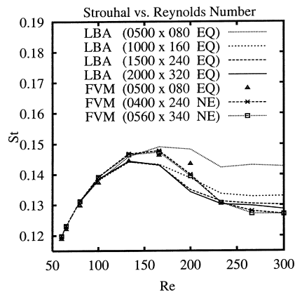
Fig. 8. Computed Strouhal numbers vs. Reynolds number for LBA and FVM on different grids.
